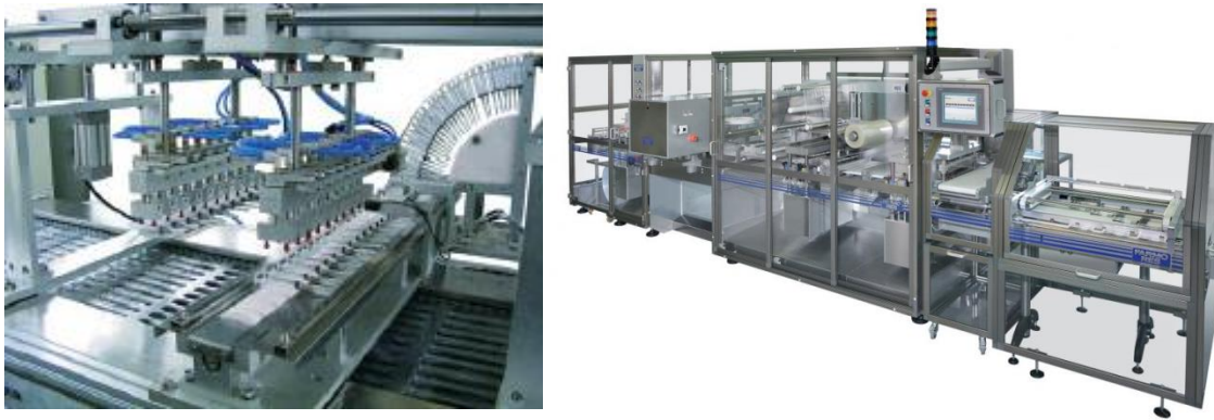
Figure 15-12. Left: internal view of a blister packaging machine (courtesy Greathealth Trexim) Right: tray pack thermoforming machine (courtesy MG America)
